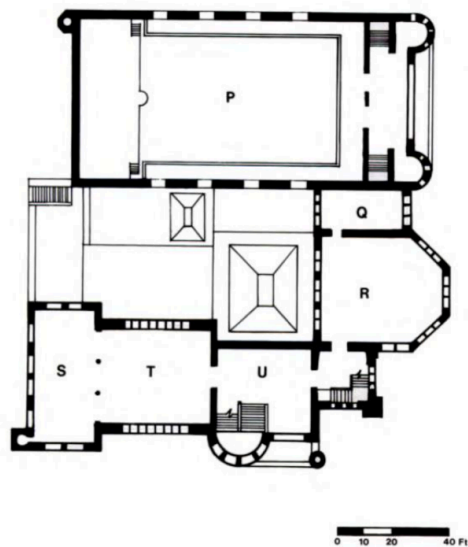
Figure 1.8 Carnegie Library, Allegheny City, second-floor plan. P = upper part of music hall, Q = apparatus room, R = lecture room, S = print room, T = art gallery, U = stair hall. Reconstructed from Library Journal 18 (August 1893): 289.
