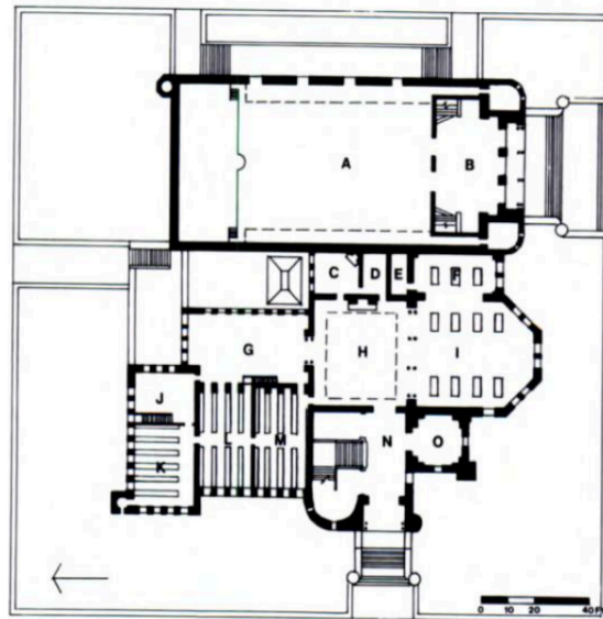
Figure 1.7 Carnegie Library, Allegheny City, first-floor plan. A = music hall, B = lobby, C = librarian's office, D = men's toilet, E = women's toilet, F = ladies' reading room, G = bibliographic room, H = delivery room, I = reading room, J = repair room, K, L, M = stack rooms, N = lobby, O = trustees' room. Redrawn from Library Journal 18 (August 1893): 289.
