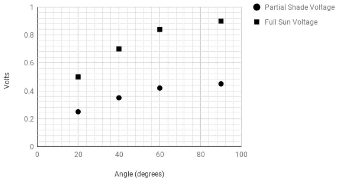
Effect of Light Angle on Voltage in Partial Shade and Full Sun
